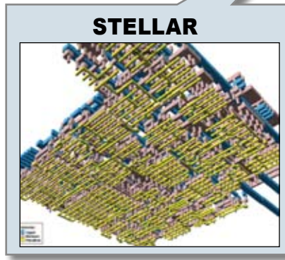
3D PHYSICS-BASED RC EXTRACTOR FOR LARGE CELLS
