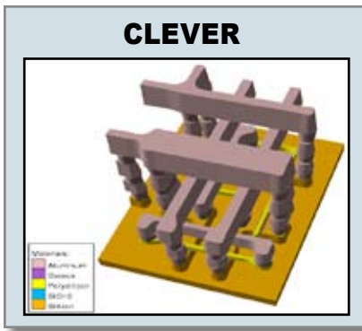
RC EXTRACTOR FOR REALISTIC 3D STRUCTURES
